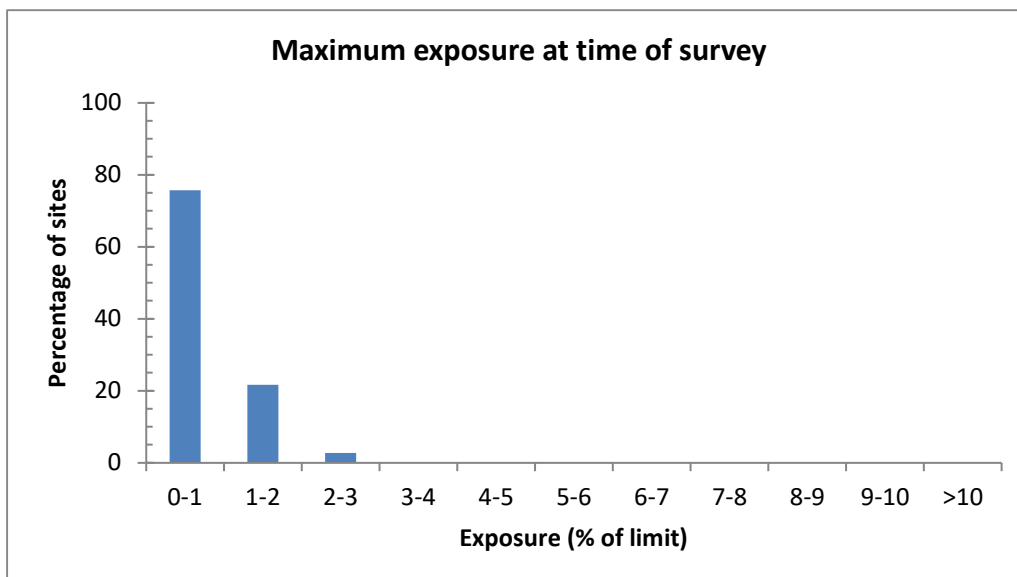
Fig 1. Histogram of maximum exposures found at the time of measurement at the 48 sites surveyed in 2019-20.
