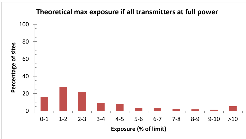
Fig 4. Histogram of theoretical maximum possible exposures for all 280 sites surveyed since 2014, if they and all other sites nearby were to transmit at full power.
