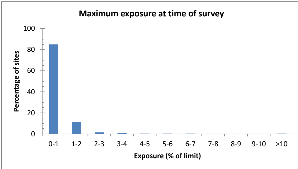
Fig 3. Histogram of maximum exposures found at the time of measurement for all 280 sites surveyed since 2014.
