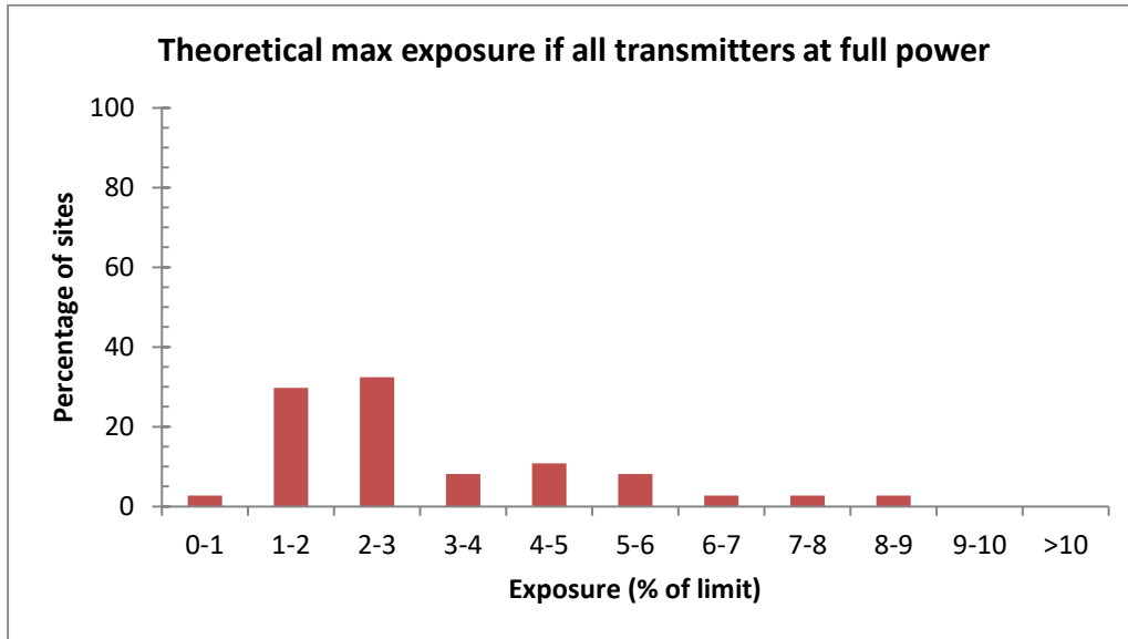
Fig 2. Histogram of theoretical maximum possible exposures at the 37 sites surveyed in 2019-20, if they and all other sites nearby were to transmit at full power.
